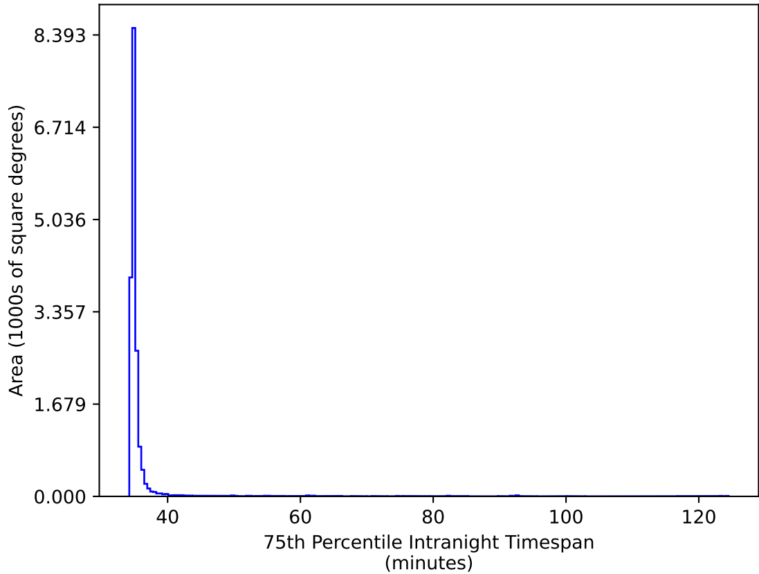
too_elab_heavy_r64_d2_gz_v3.4_10yrs WFD gr bands: 75th Percentile Intranight Timespan
