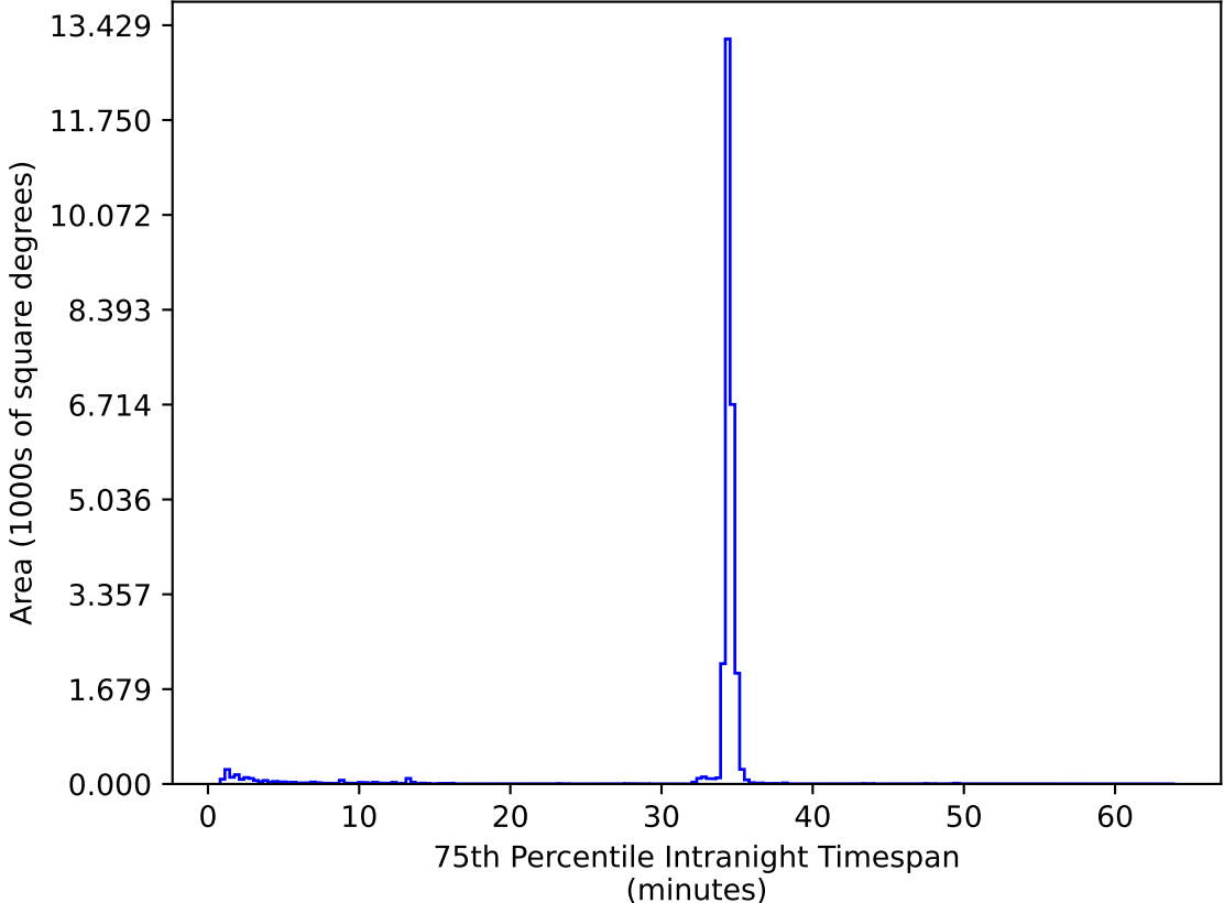
too_elab_heavy_r64_d2_gz_v3.4_10yrs All sky zy bands: 75th Percentile Intranight Timespan
