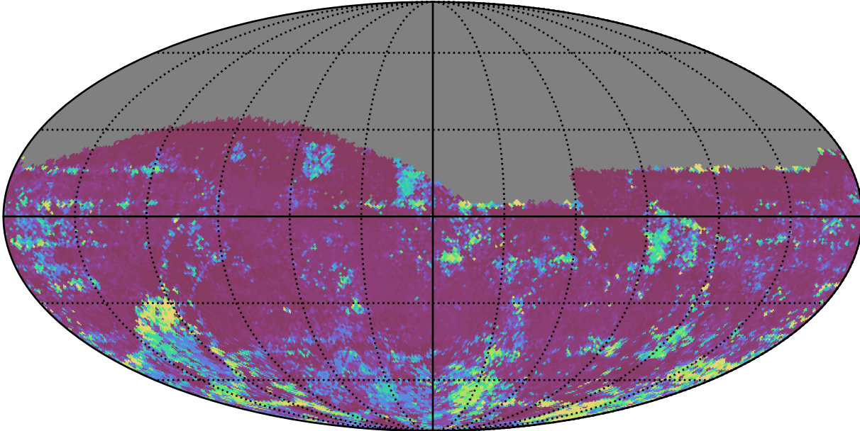
too_elab_heavy_r64_d2_gz_v3.4_10yrs All sky z band: 75th Percentile Intranight Timespan
