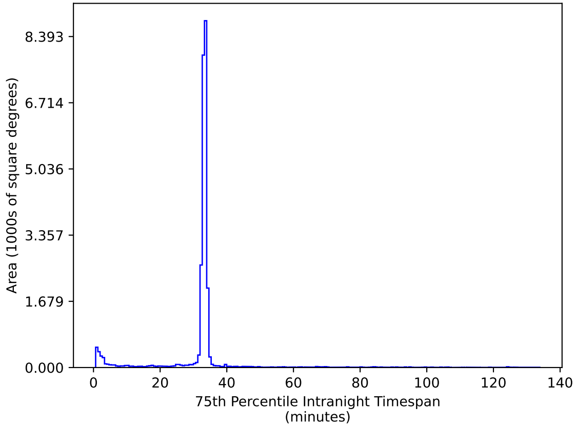
too_elab_heavy_r64_d2_gz_v3.4_10yrs All sky ug bands: 75th Percentile Intranight Timespan
