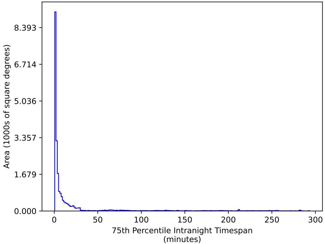
too_elab_heavy_r64_d2_gz_v3.4_10yrs All sky u band: 75th Percentile Intranight Timespan
