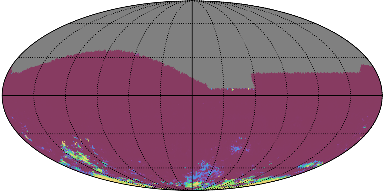
too_elab_heavy_r64_d2_gz_v3.4_10yrs All sky ri bands: 75th Percentile Intranight Timespan
