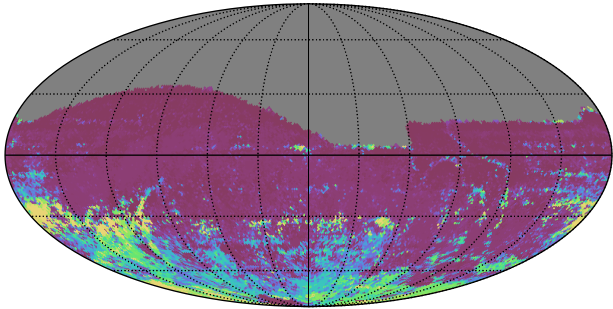
too_elab_heavy_r64_d2_gz_v3.4_10yrs All sky r band: 75th Percentile Intranight Timespan
