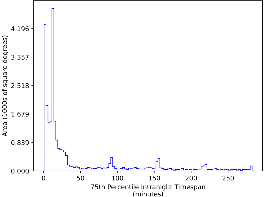
too_elab_heavy_r64_d2_gz_v3.4_10yrs All sky r band: 75th Percentile Intranight Timespan
