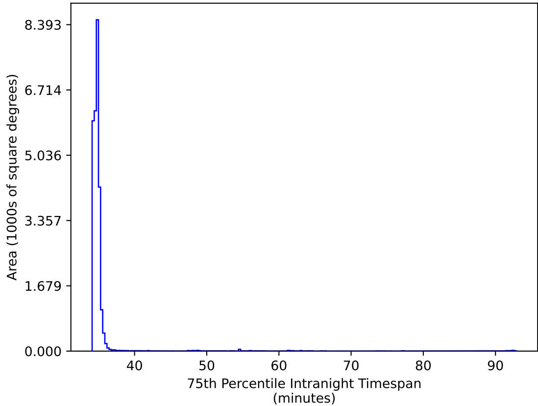
too_elab_heavy_r64_d2_gz_v3.4_10yrs All sky iz bands: 75th Percentile Intranight Timespan
