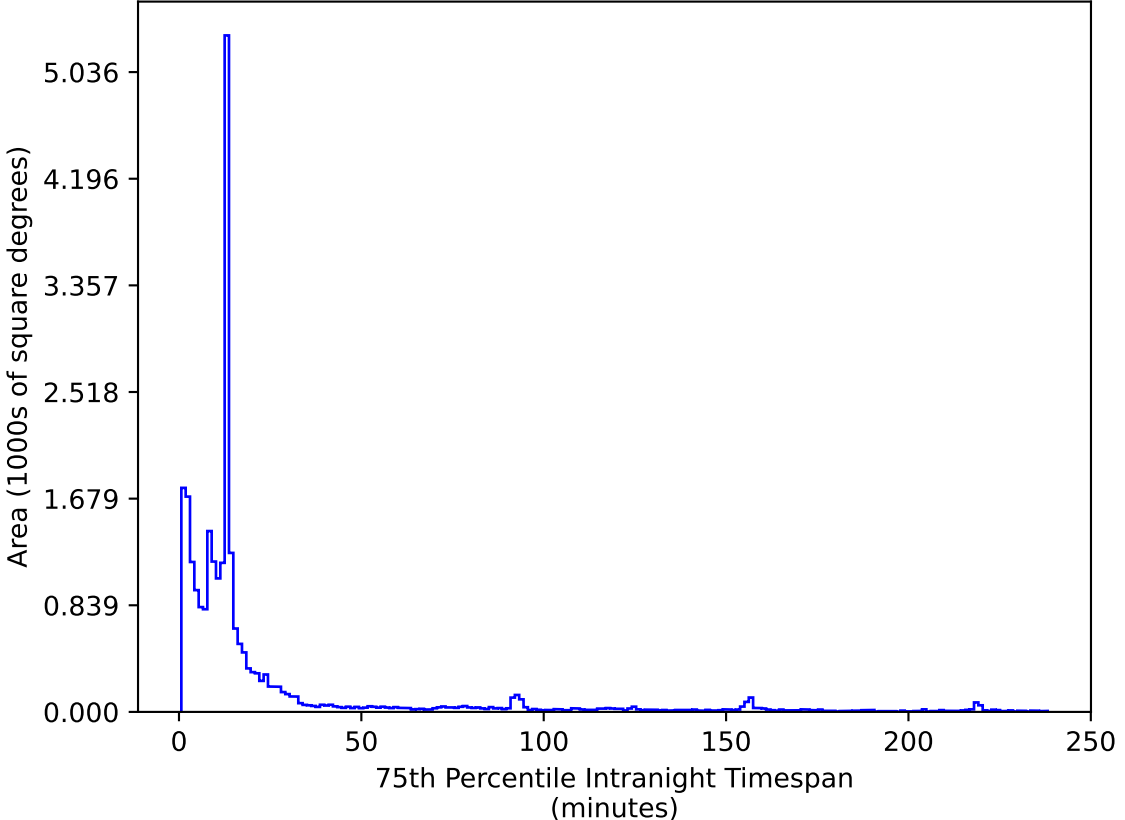
too_elab_heavy_r64_d2_gz_v3.4_10yrs All sky i band: 75th Percentile Intranight Timespan
