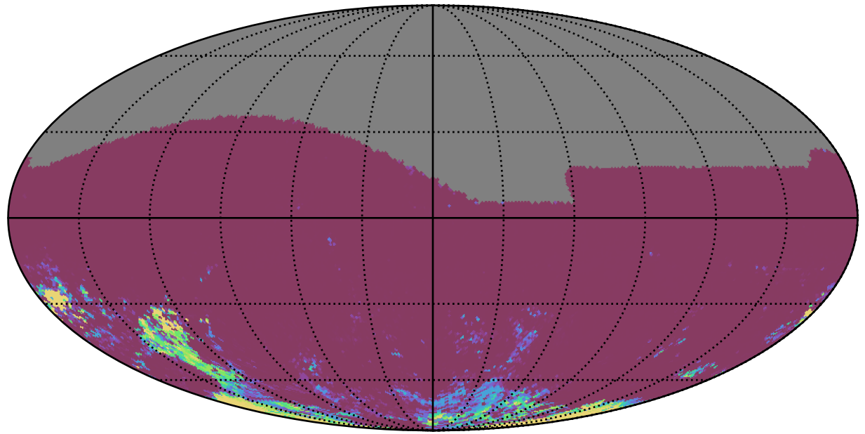
too_elab_heavy_r64_d2_gz_v3.4_10yrs All sky gr bands: 75th Percentile Intranight Timespan
