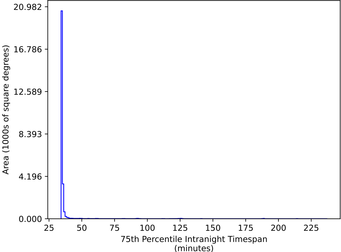
too_elab_heavy_r64_d2_gz_v3.4_10yrs All sky gr bands: 75th Percentile Intranight Timespan
