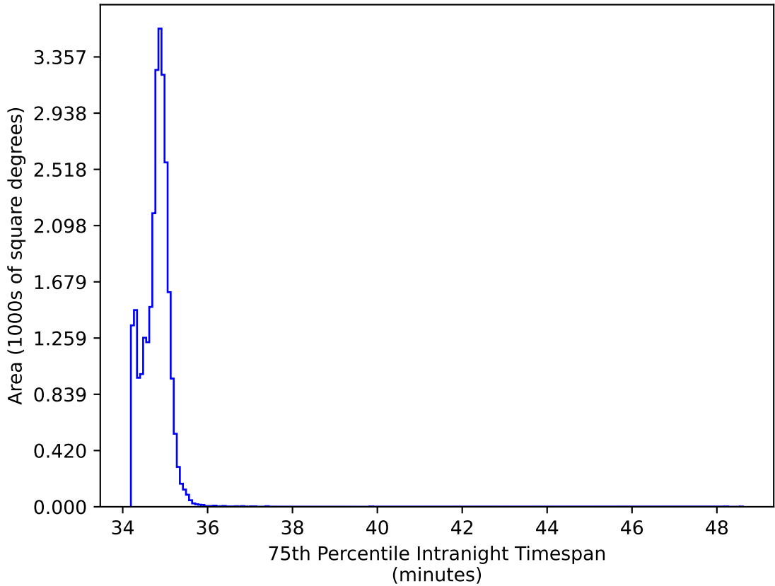
too_elab_heavy_r64_d2_gz_v3.4_10yrs All sky: 75th Percentile Intranight Timespan
