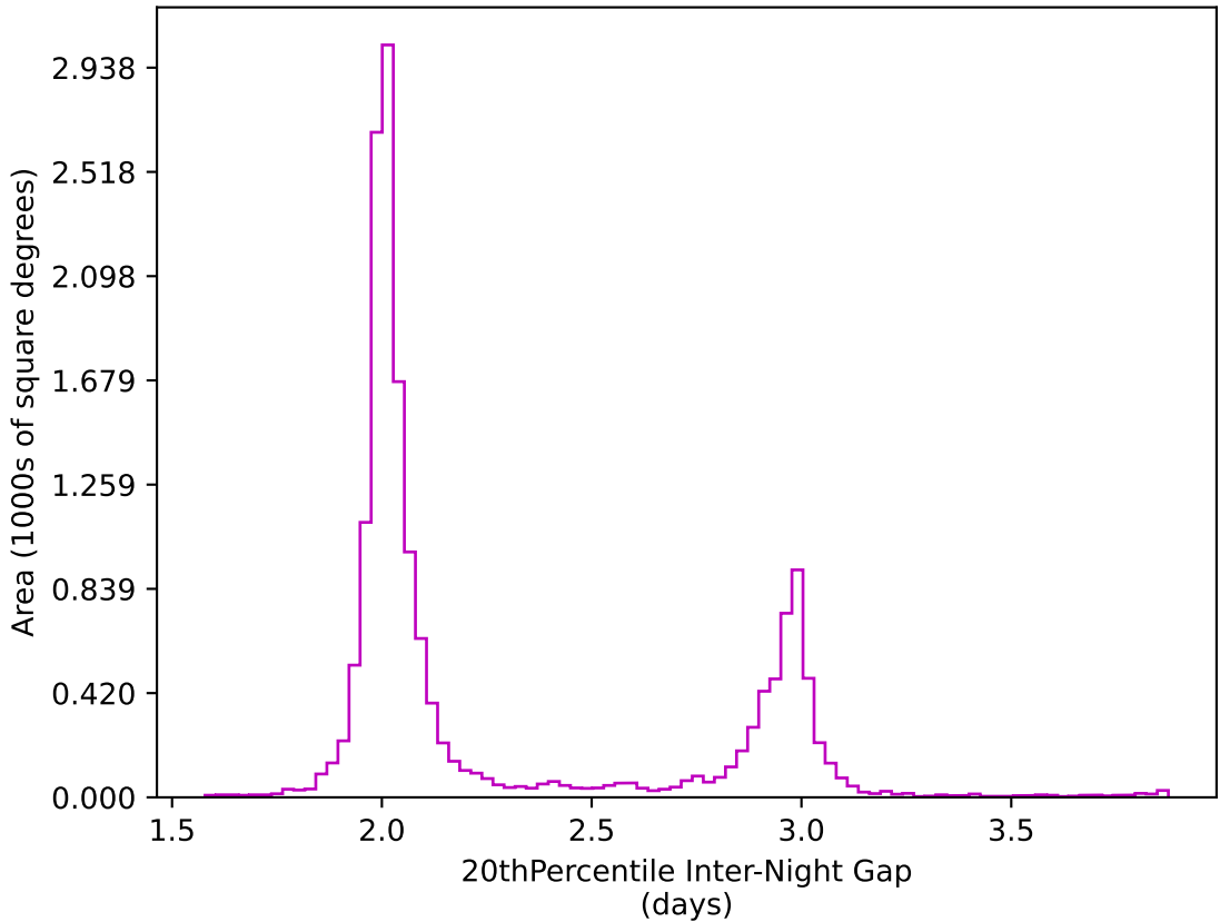
too_elab_heavy_r64_d2_gz_v3.4_10yrs WFD z band: 20thPercentile Inter-Night Gap
