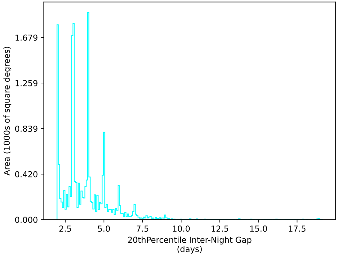
too_elab_heavy_r64_d2_gz_v3.4_10yrs WFD u band: 20thPercentile Inter-Night Gap
