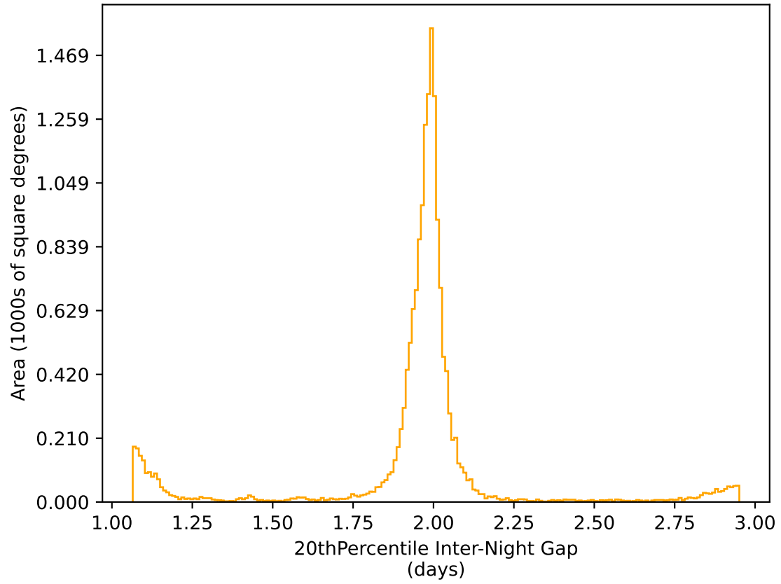
too_elab_heavy_r64_d2_gz_v3.4_10yrs WFD r band: 20thPercentile Inter-Night Gap
