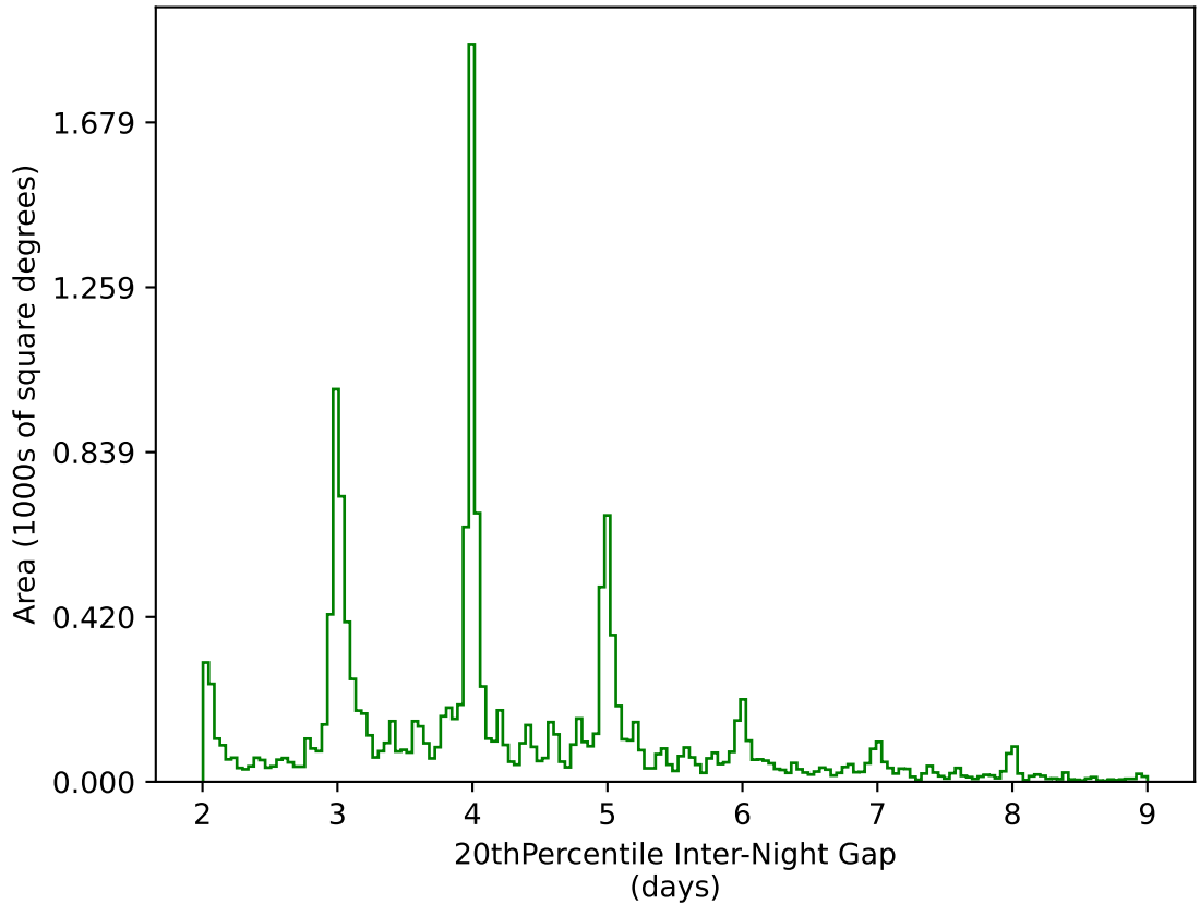
too_elab_heavy_r64_d2_gz_v3.4_10yrs WFD g band: 20thPercentile Inter-Night Gap
