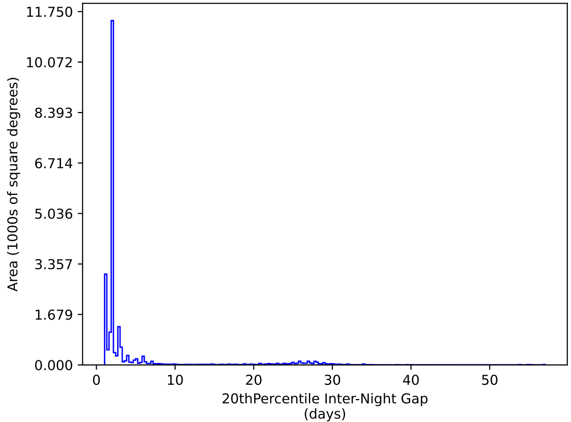
too_elab_heavy_r64_d2_gz_v3.4_10yrs All sky y band: 20thPercentile Inter-Night Gap
