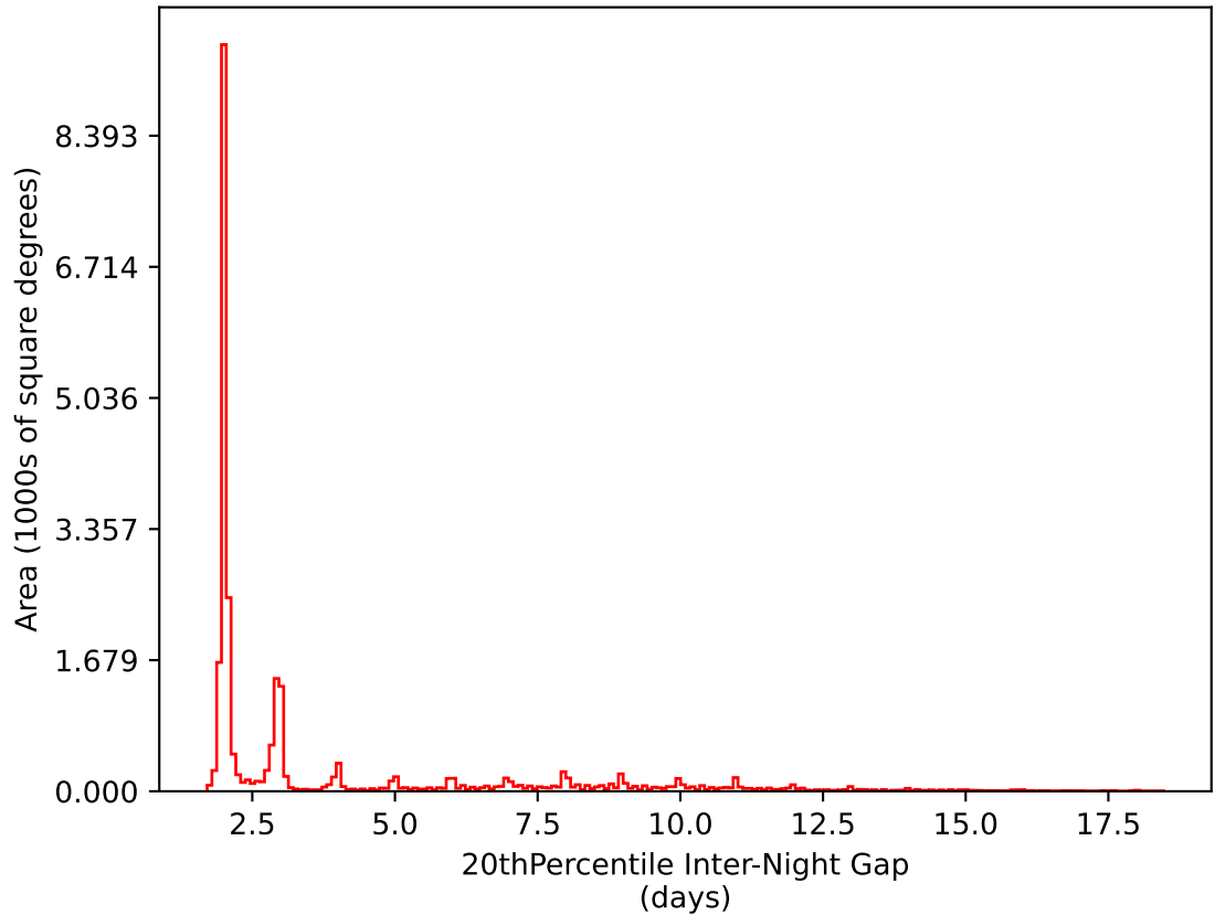
too_elab_heavy_r64_d2_gz_v3.4_10yrs All sky i band: 20thPercentile Inter-Night Gap
