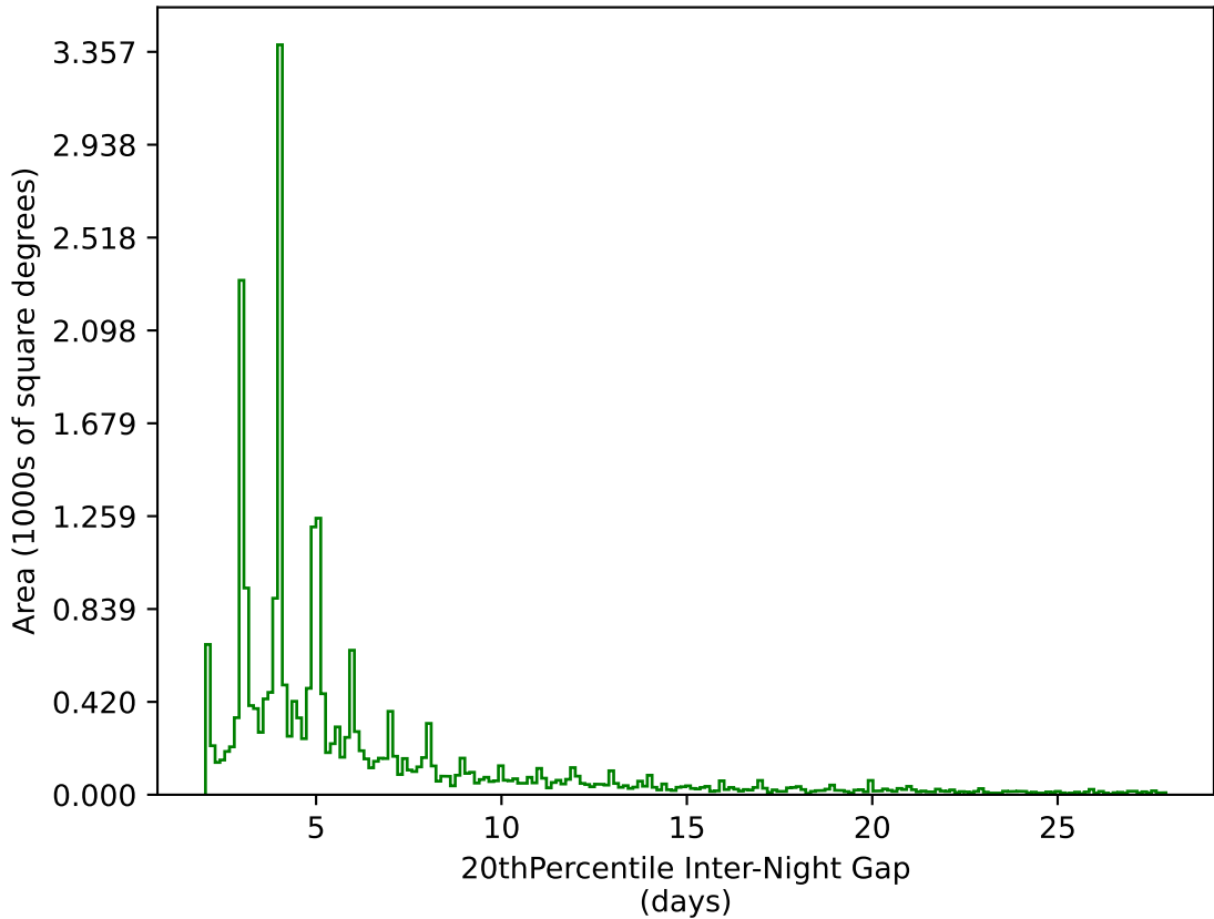
too_elab_heavy_r64_d2_gz_v3.4_10yrs All sky g band: 20thPercentile Inter-Night Gap
