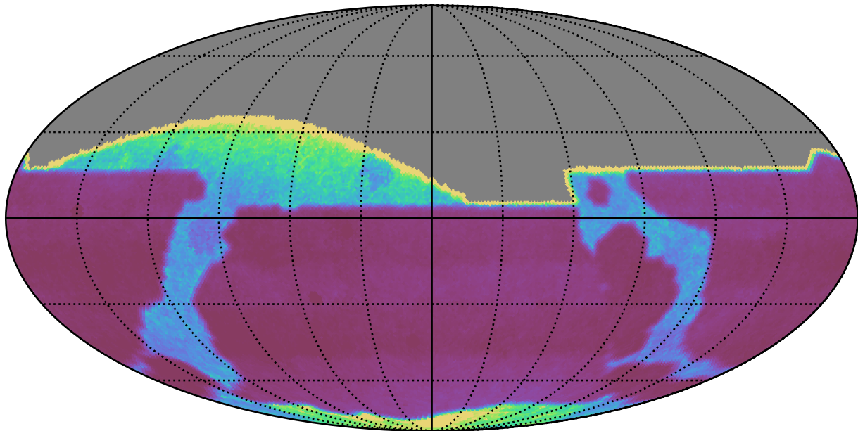
too_elab_heavy_r64_d2_gz_v3.4_10yrs : properMotion
