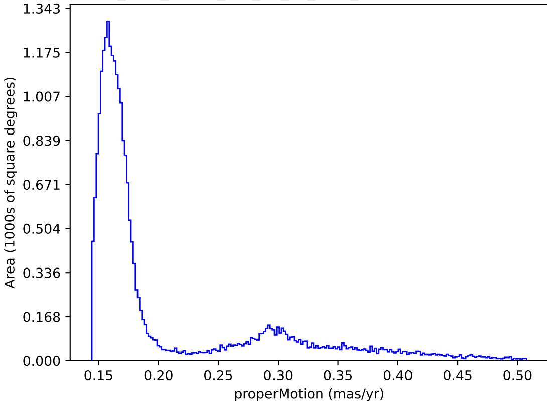
too_elab_heavy_r64_d2_gz_v3.4_10yrs : properMotion
