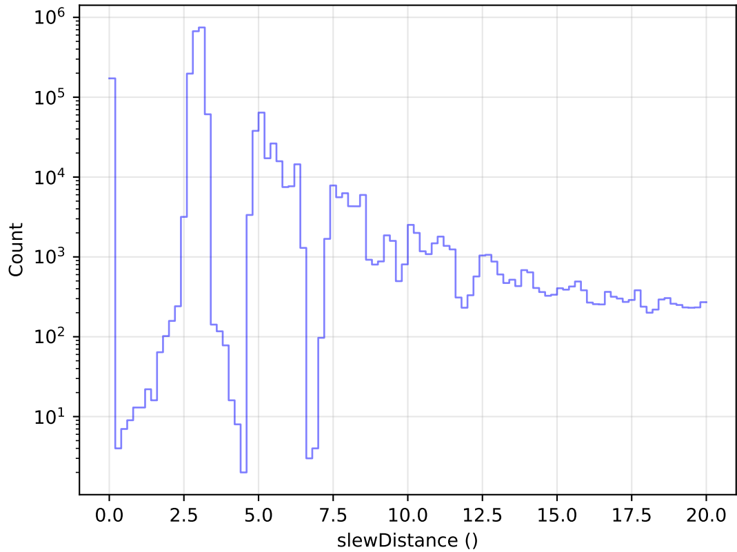
too_elab_heavy_r64_d2_gz_v3.4_10yrs All visits: Zoom Slew Distance Histogram
