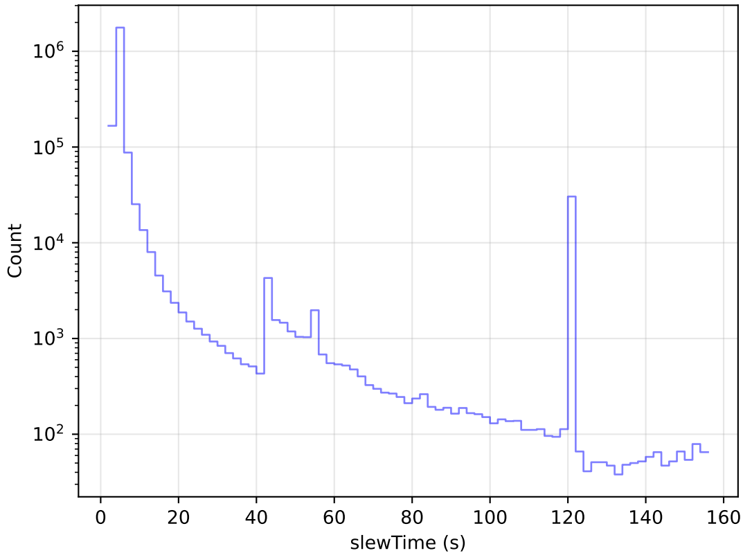
too_elab_heavy_r64_d2_gz_v3.4_10yrs All visits: Slew Time Histogram
