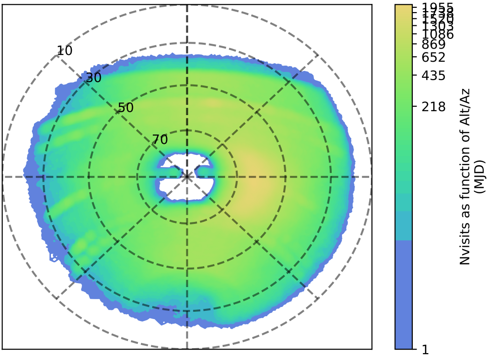
too_elab_heavy_r64_d2_gz_v3.4_10yrs y: Nvisits as function of Alt/Az
