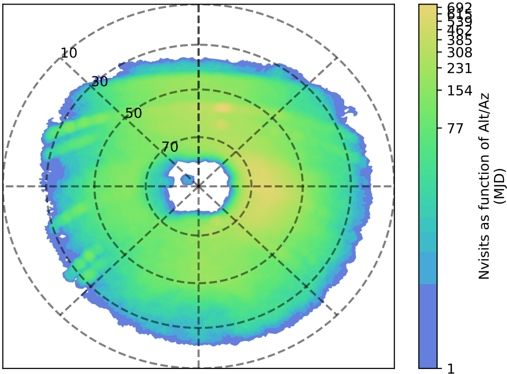
too_elab_heavy_r64_d2_gz_v3.4_10yrs u: Nvisits as function of Alt/Az
