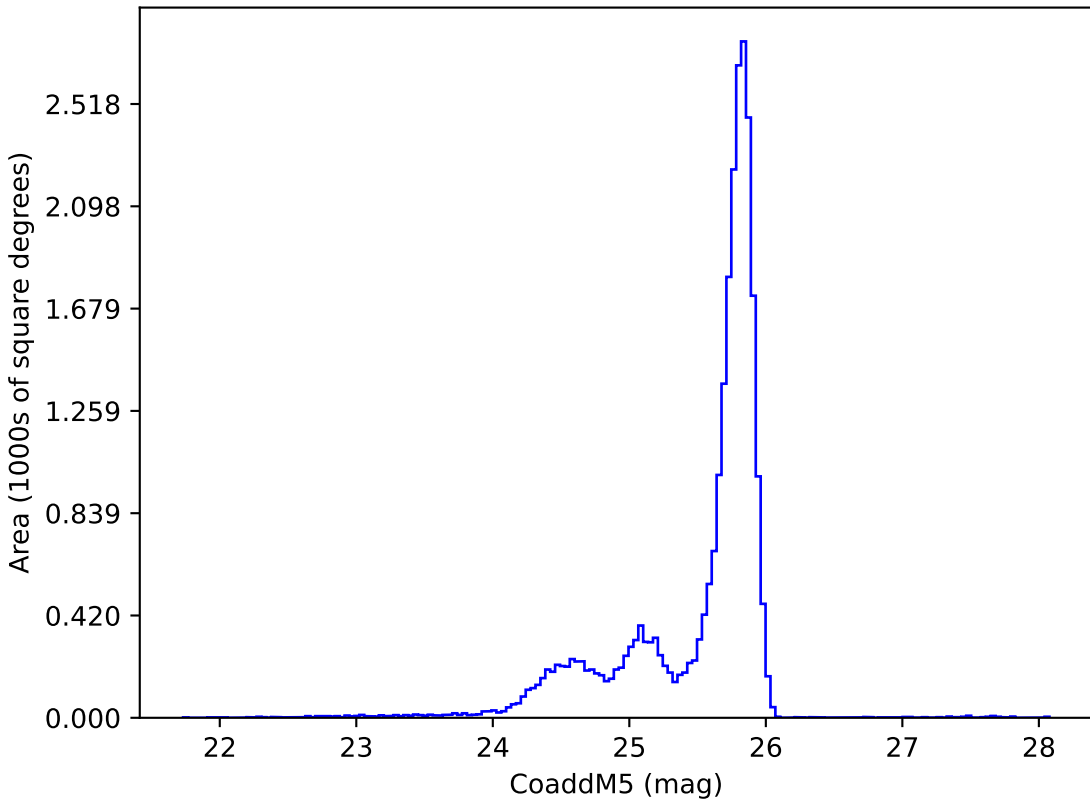
too_elab_heavy_r64_d2_gz_v3.4_10yrs z: CoaddM5
