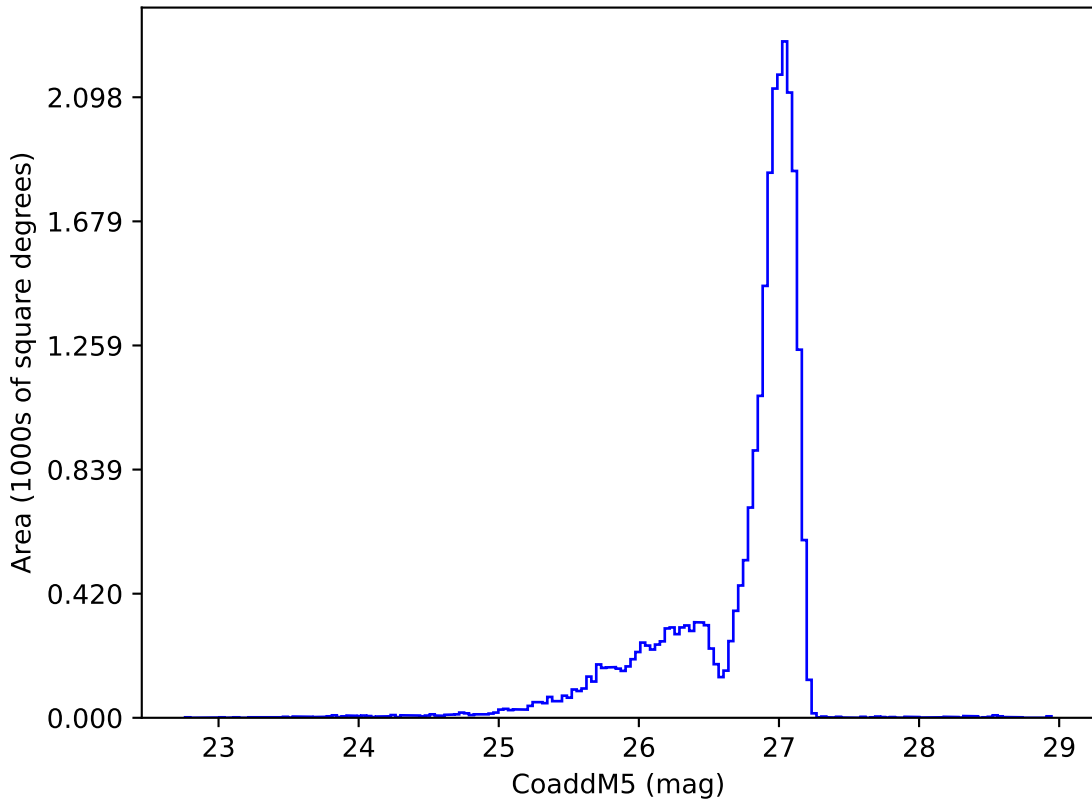
too_elab_heavy_r64_d2_gz_v3.4_10yrs r: CoaddM5
