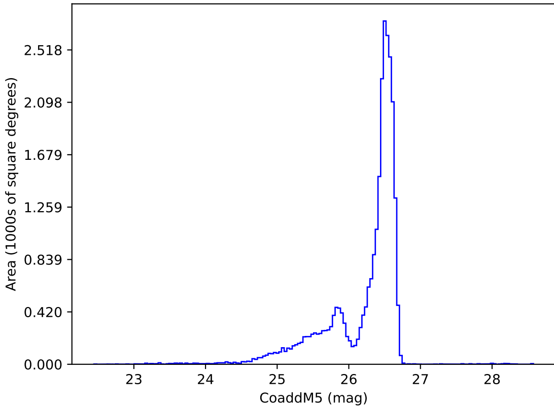
too_elab_heavy_r64_d2_gz_v3.4_10yrs i: CoaddM5
