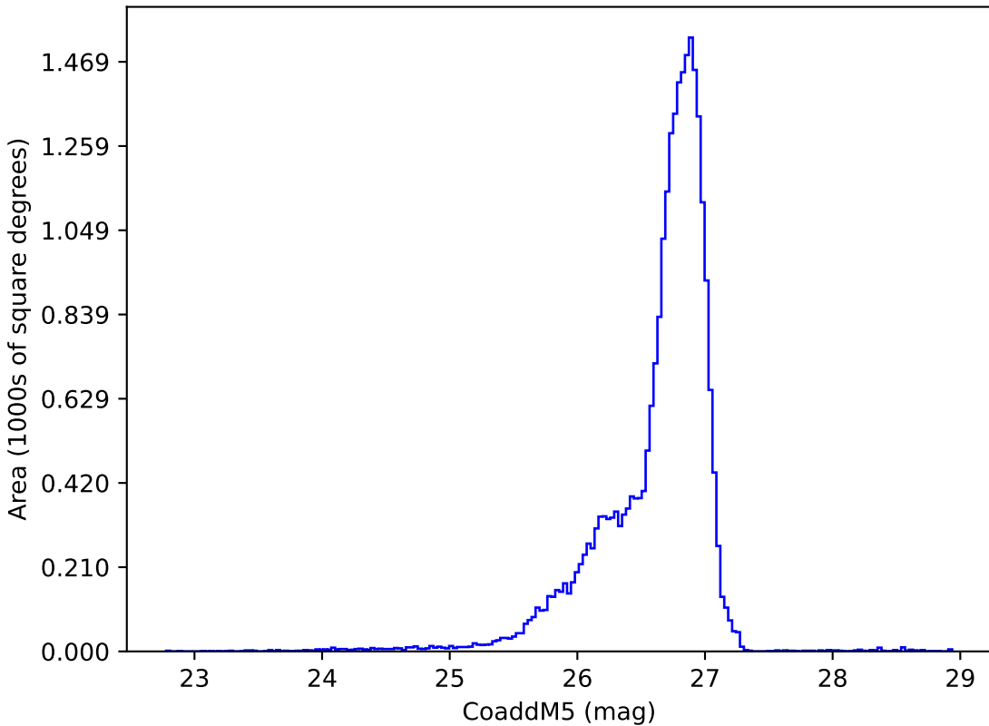
too_elab_heavy_r64_d2_gz_v3.4_10yrs g: CoaddM5
