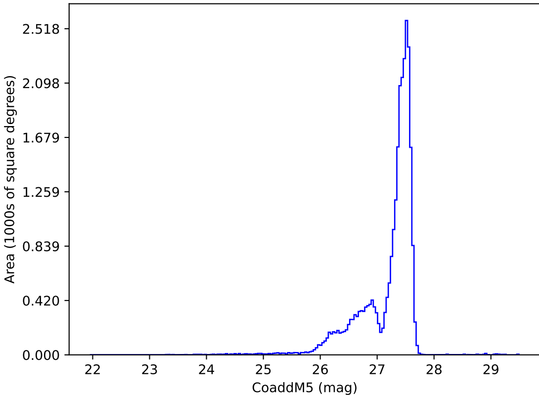
too_elab_heavy_r64_d2_gz_v3.4_10yrs : CoaddM5
