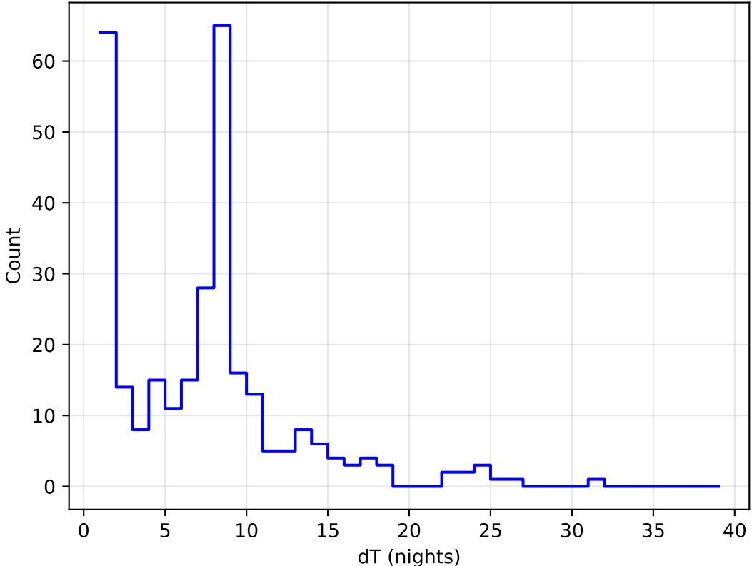
too_elab_heavy_r64_d2_gz_v3.4_10yrs all bands: DD:XMM_LSS Delta Nights Histogram
