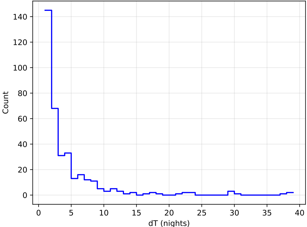
too_elab_heavy_r64_d2_gz_v3.4_10yrs all bands: DD:WFD Delta Nights Histogram
