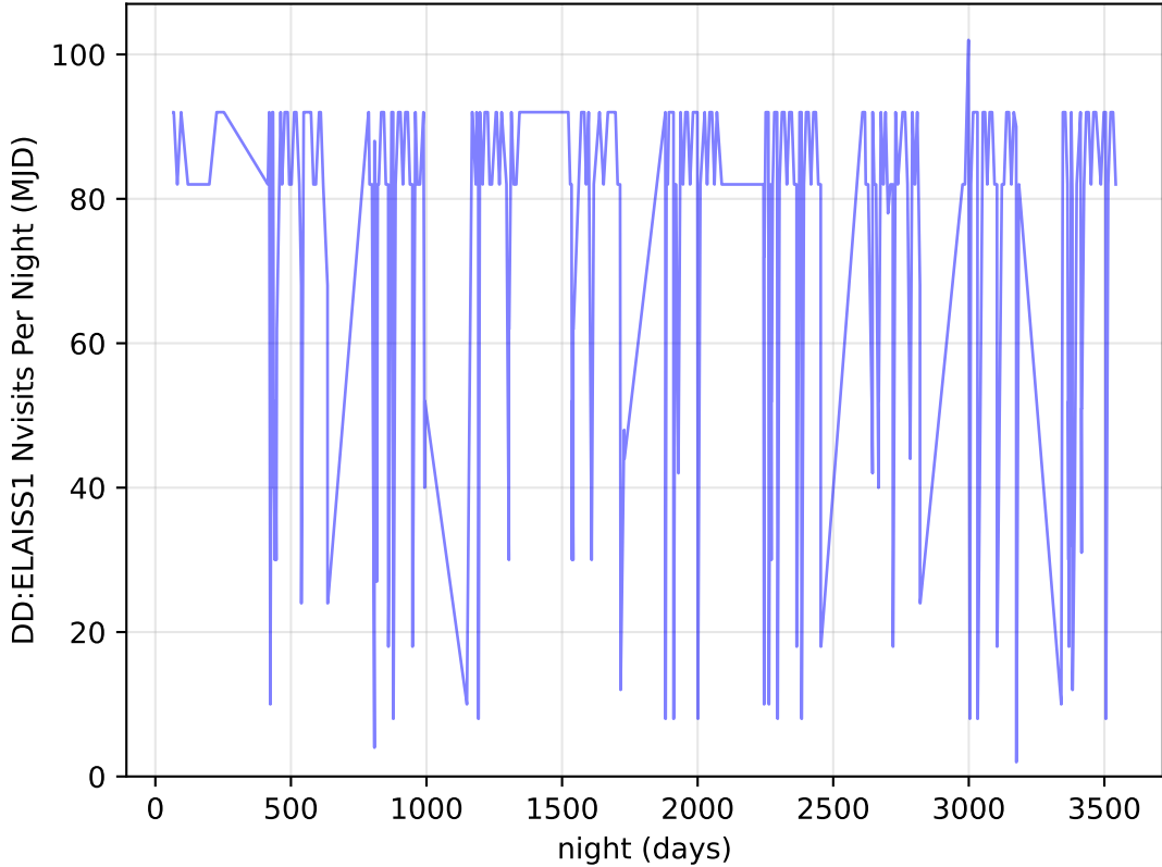
too_elab_heavy_r64_d2_gz_v3.4_10yrs all bands: DD:ELAISS1 Nvisits Per Night
