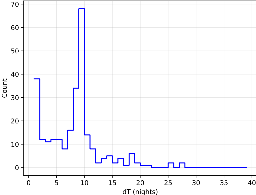
too_elab_heavy_r64_d2_gz_v3.4_10yrs all bands: DD:ELAISS1 Delta Nights Histogram
