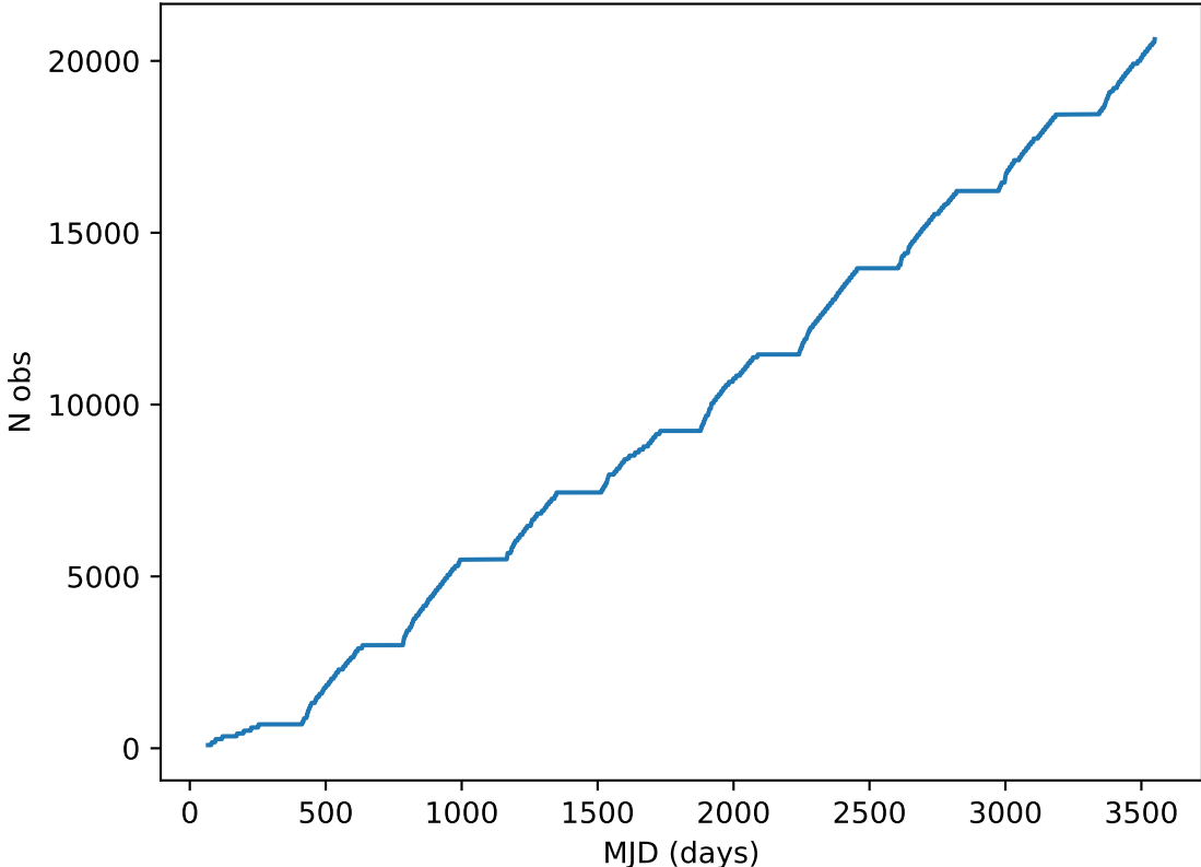
too_elab_heavy_r64_d2_gz_v3.4_10yrs all bands: DD:ELAISS1 Cumulative NVisits
