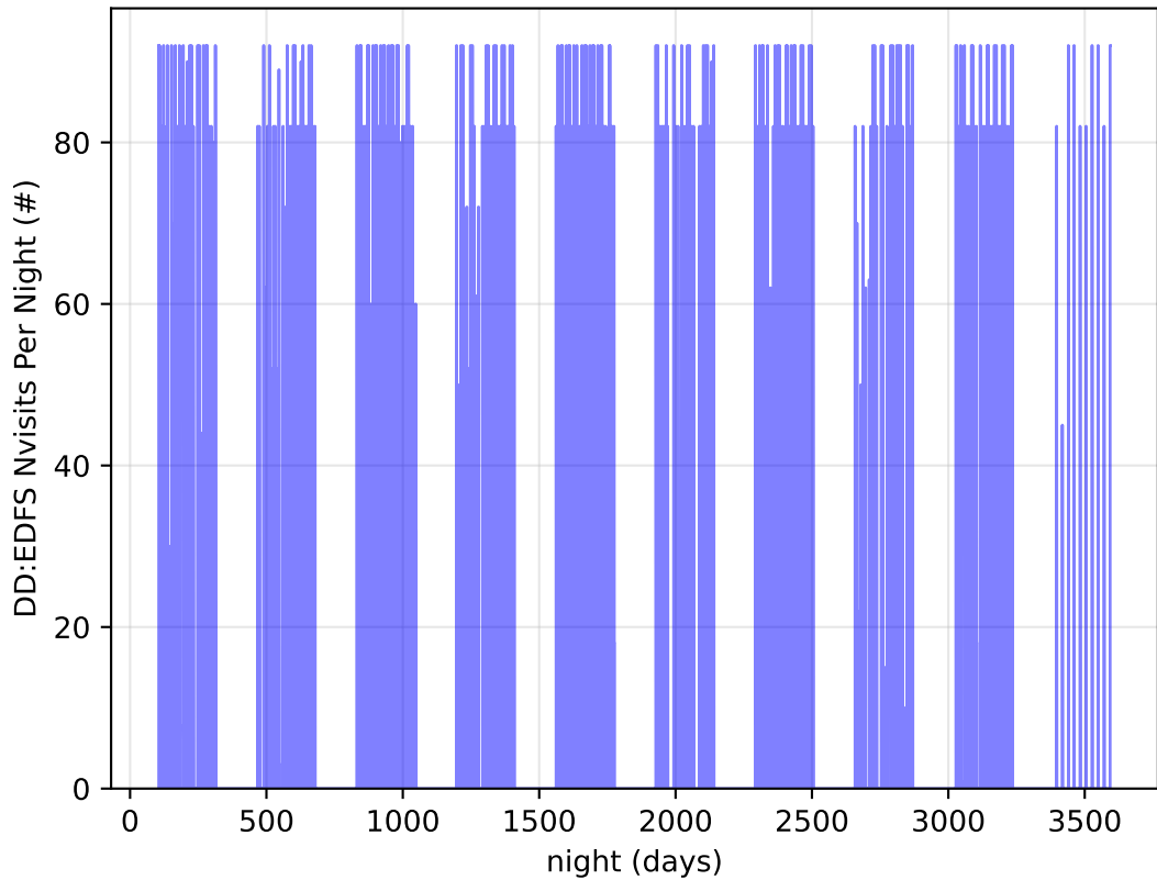
too_elab_heavy_r64_d2_gz_v3.4_10yrs all bands: DD:EDFS Nvisits Per Night
