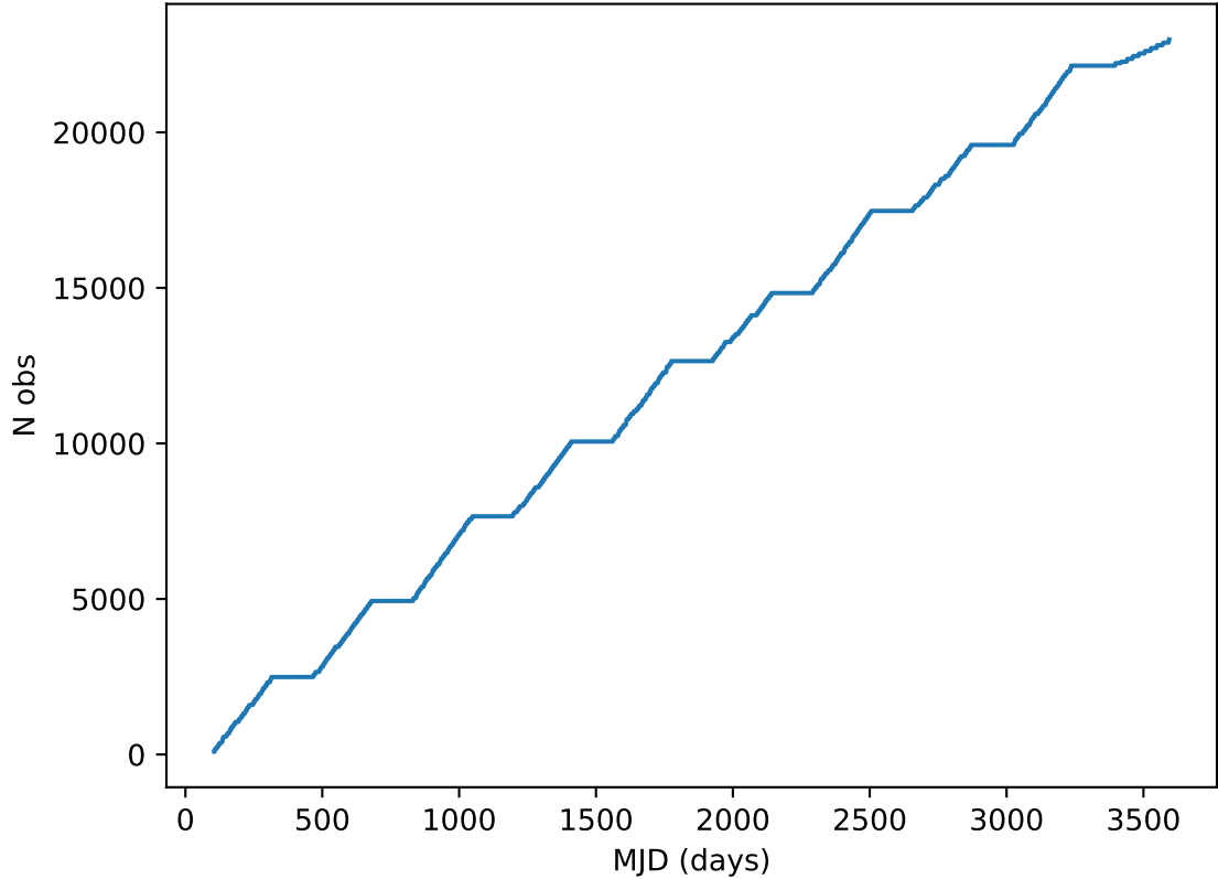
too_elab_heavy_r64_d2_gz_v3.4_10yrs all bands: DD:EDFS Cumulative NVisits
