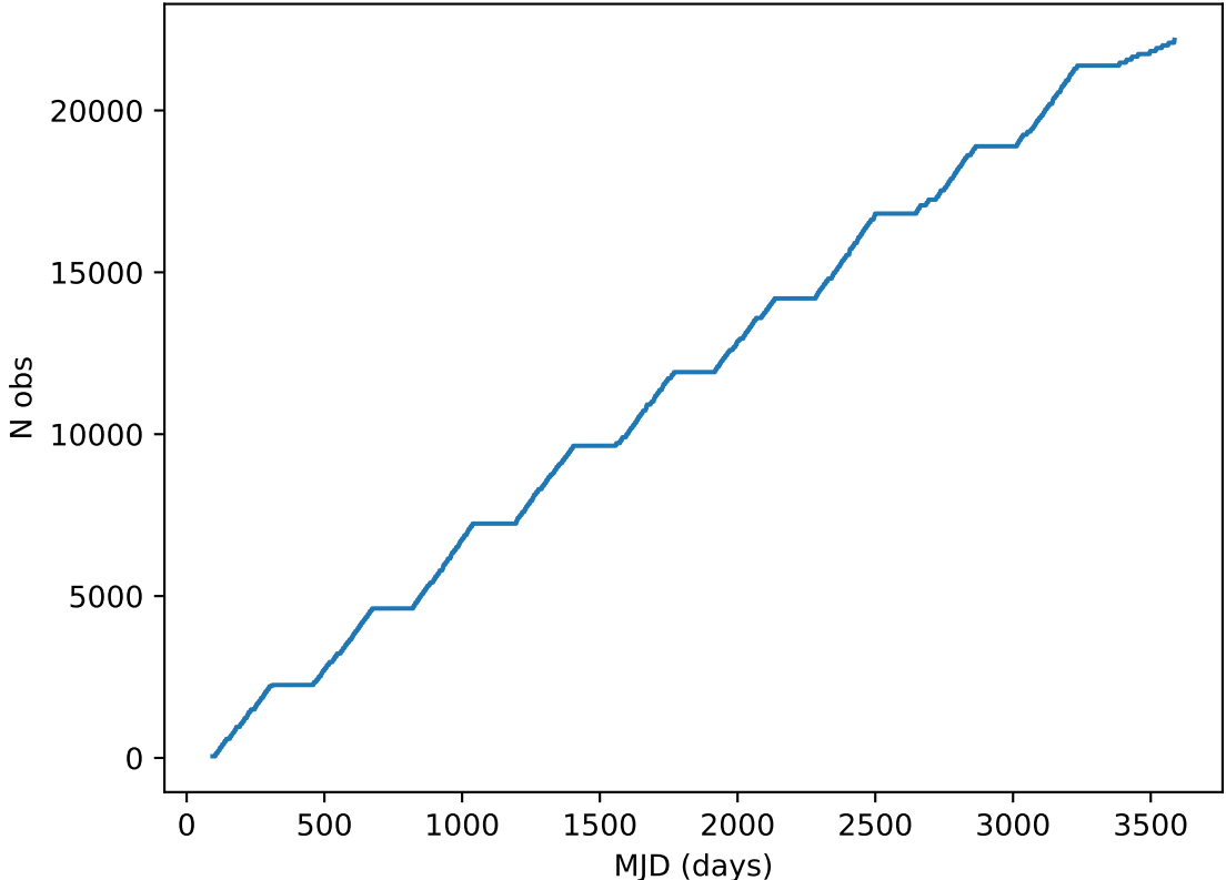
too_elab_heavy_r64_d2_gz_v3.4_10yrs all bands: DD:ECDFS Cumulative NVisits
