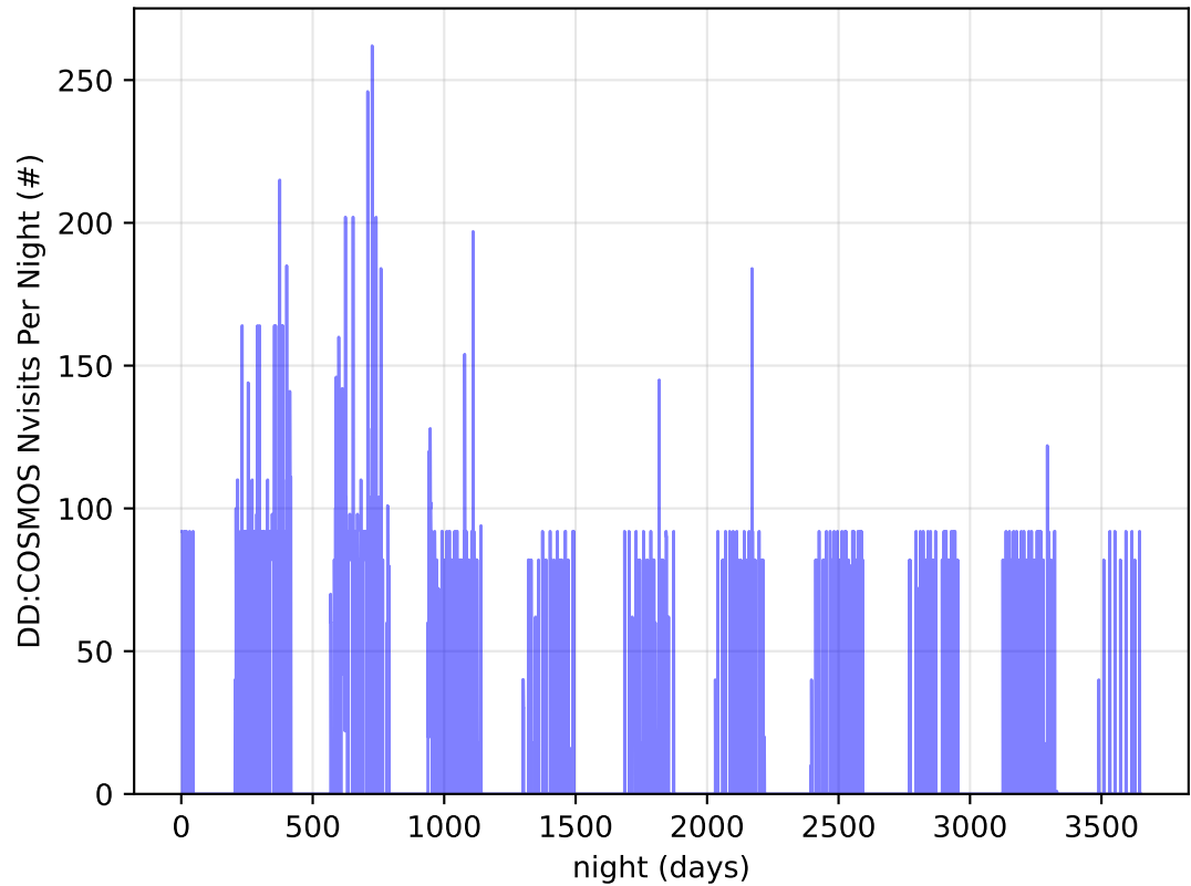
too_elab_heavy_r64_d2_gz_v3.4_10yrs all bands: DD: COSMOS Nvisits Per Night
