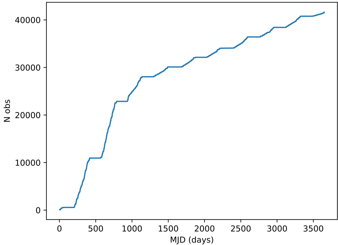
too_elab_heavy_r64_d2_gz_v3.4_10yrs all bands: DD:COSMOS Cumulative NVisits
