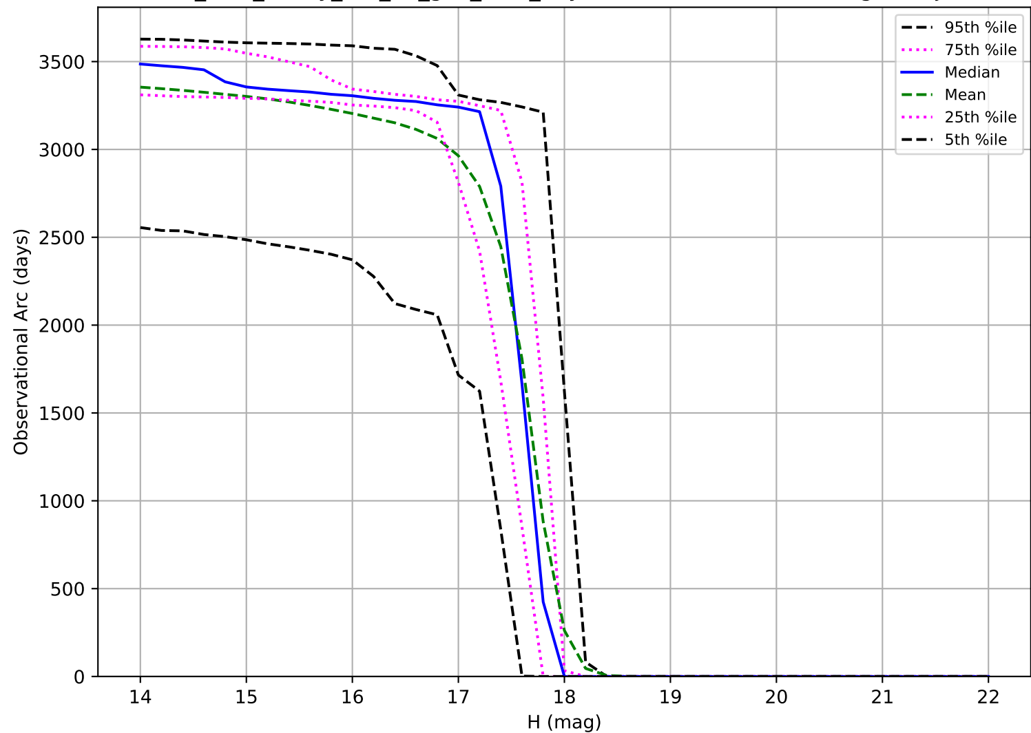
too_elab_heavy_r64_d2_griz_v3.4_10yrs: Observational Arc Length Trojan
