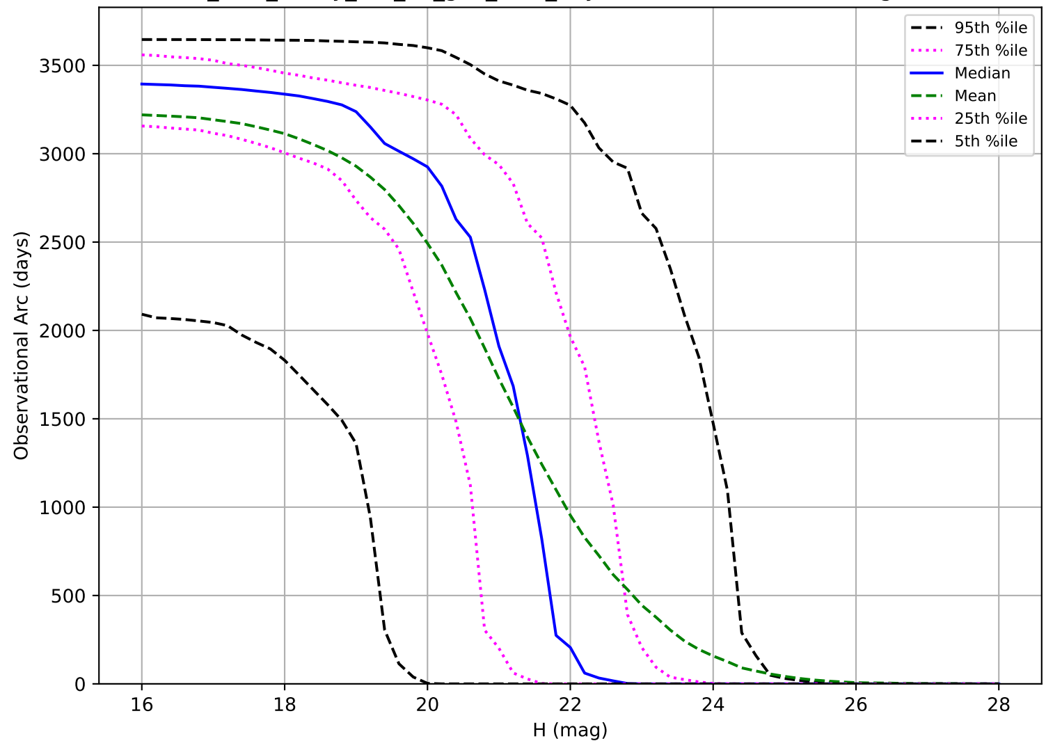
too_elab_heavy_r64_d2_griz_v3.4_10yrs: Observational Arc Length PHA
