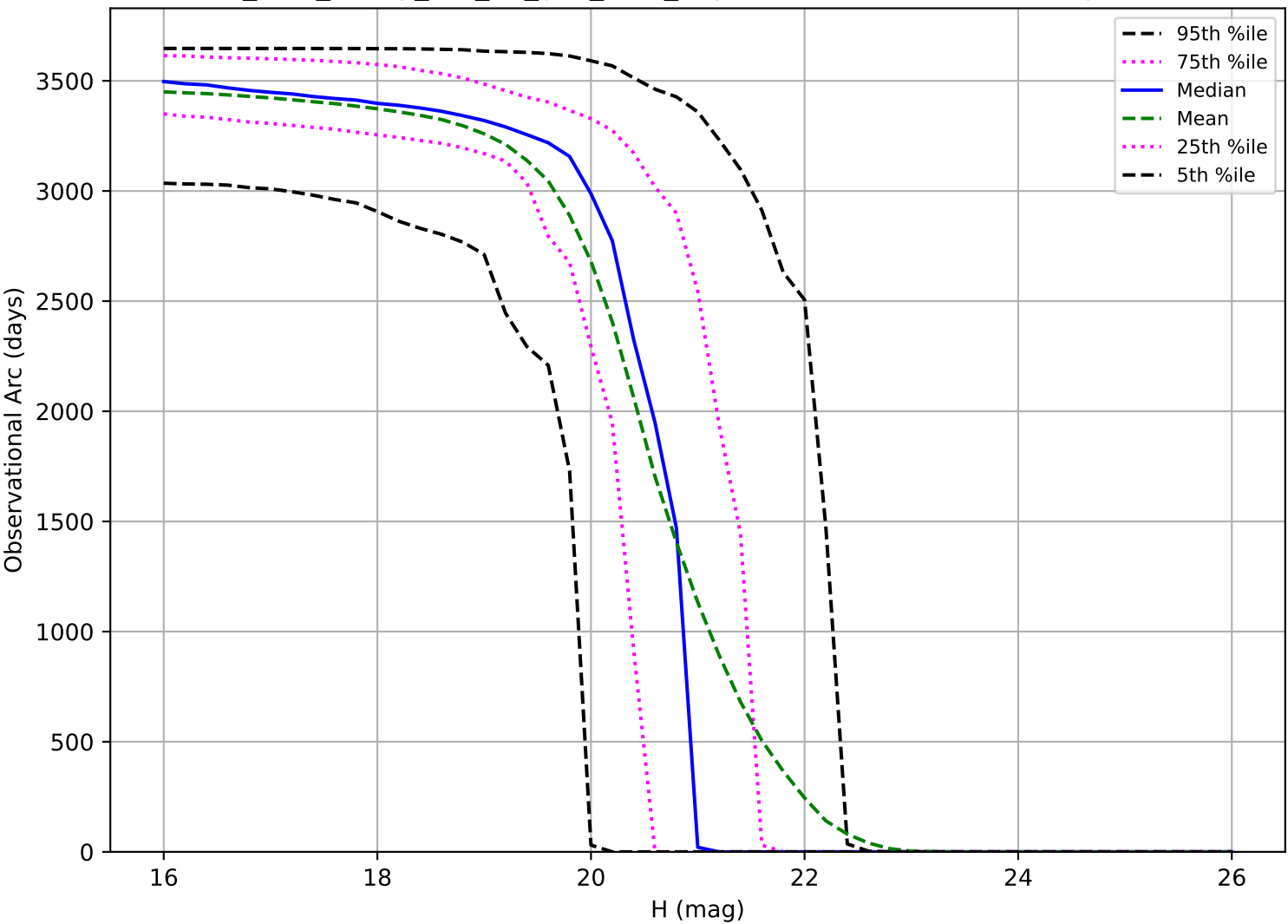
too_elab_heavy_r64_d2_griz_v3.4_10yrs: Observational Arc Length MBA
