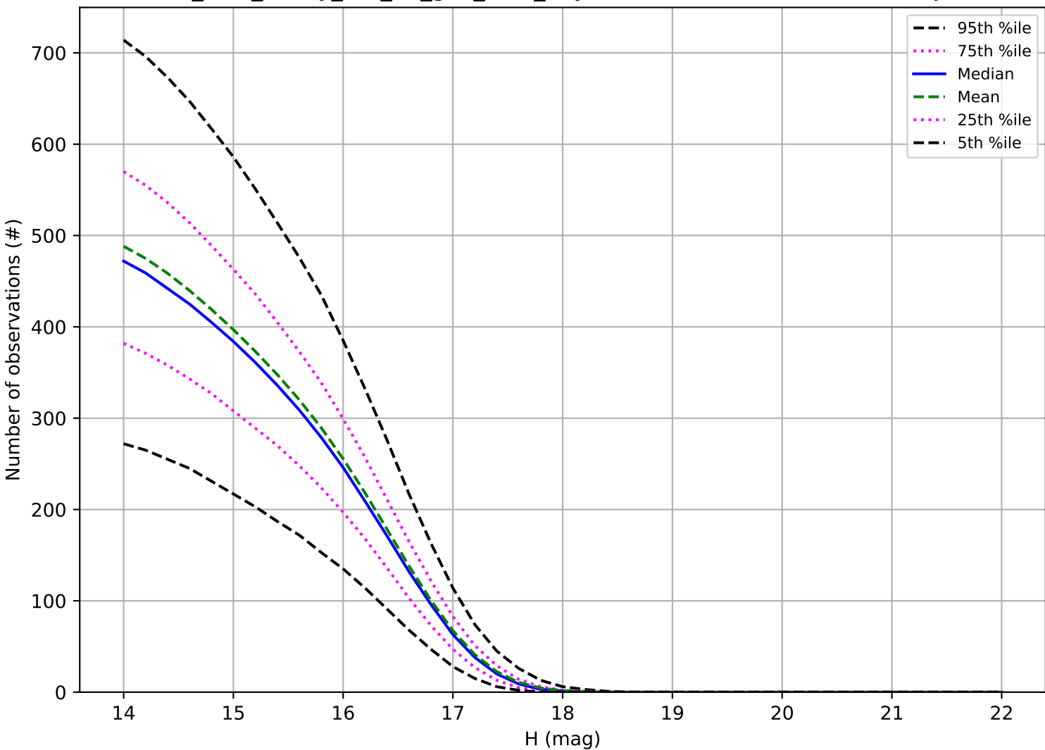
too_elab_heavy_r64_d2_griz_v3.4_10yrs: Number of observations Trojan
