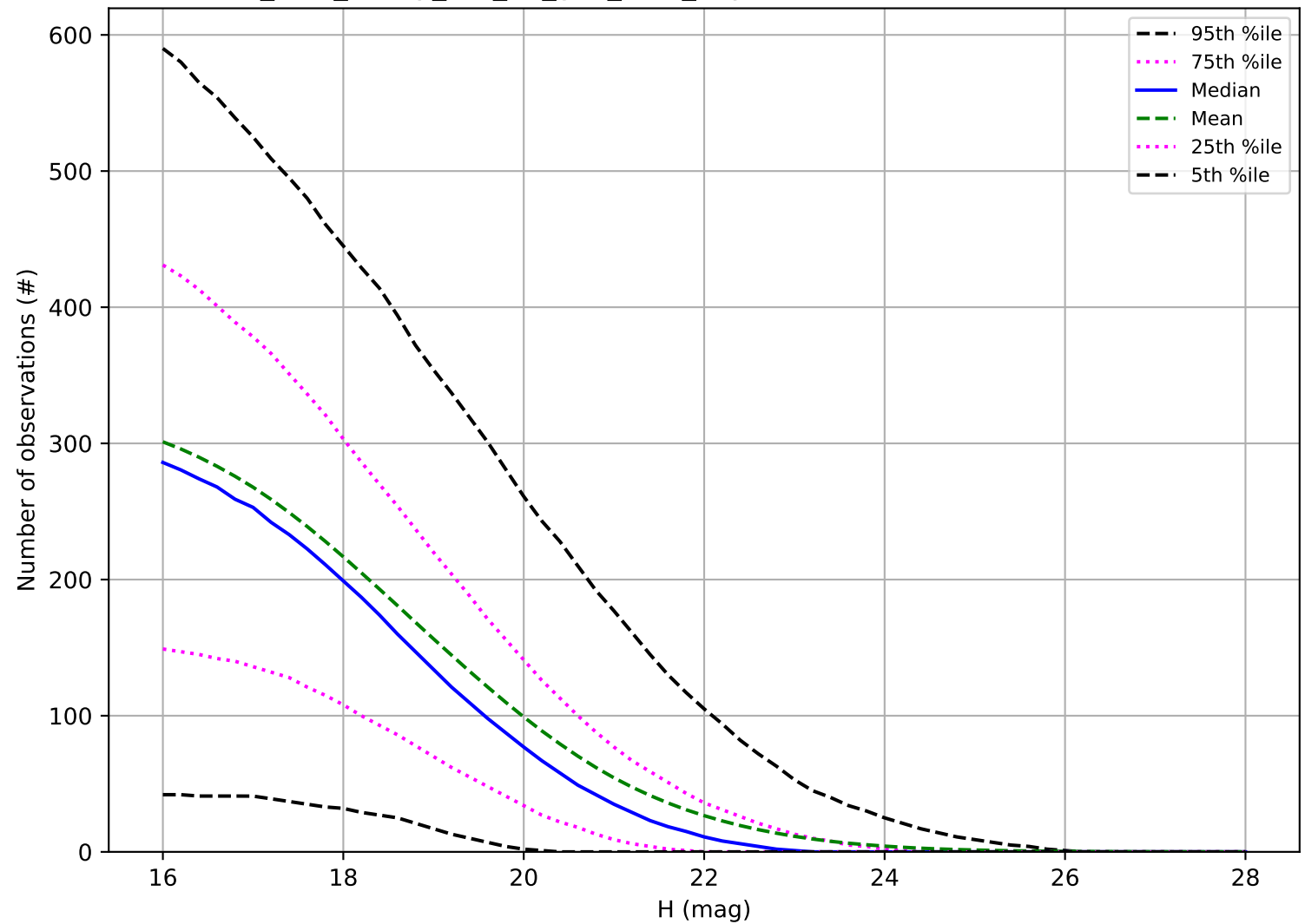
too_elab_heavy_r64_d2_griz_v3.4_10yrs: Number of observations PHA
