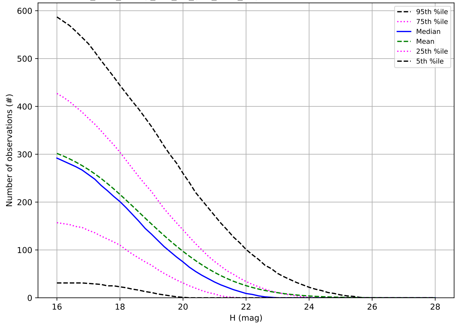
too_elab_heavy_r64_d2_griz_v3.4_10yrs: Number of observations NEO
