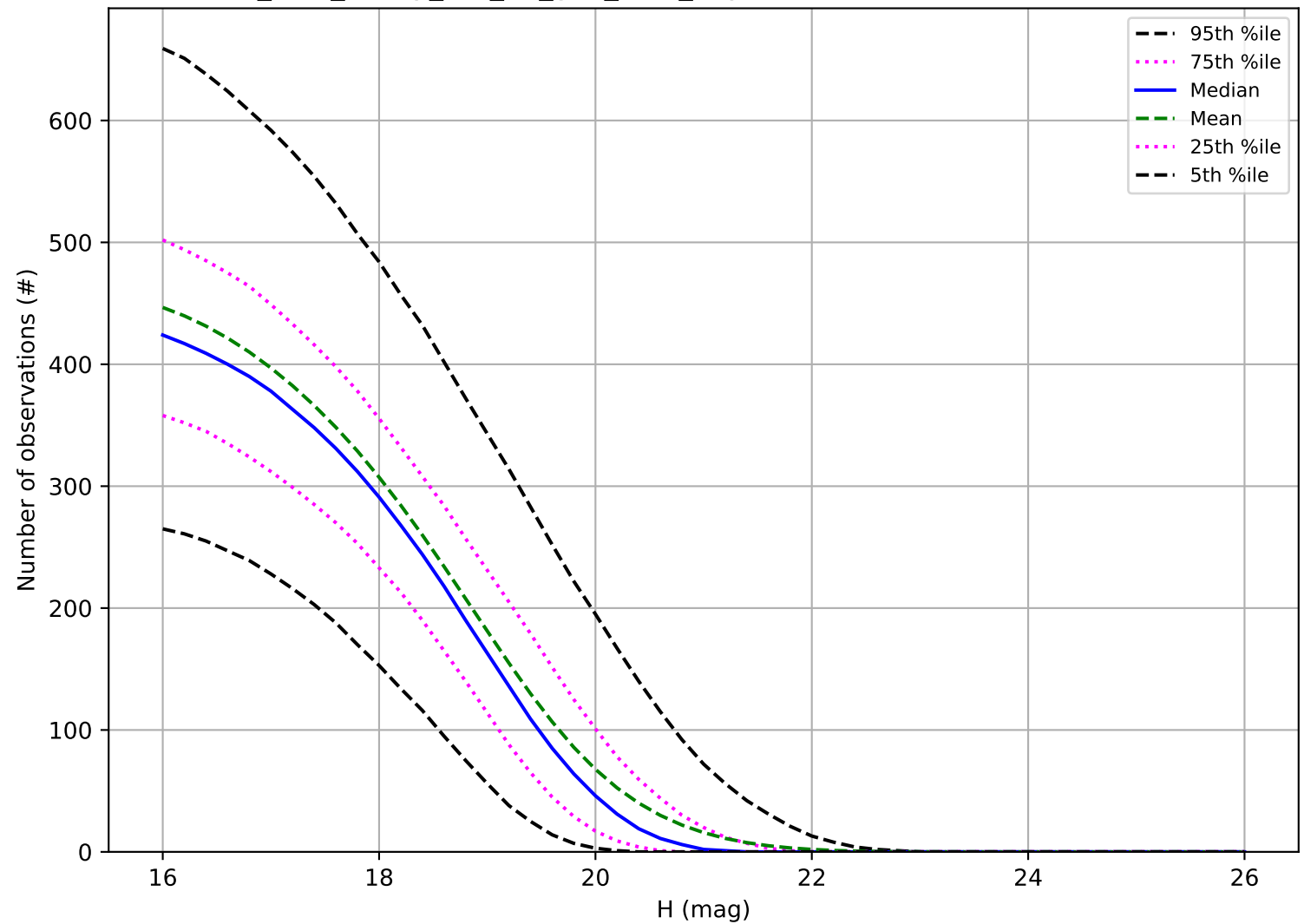
too_elab_heavy_r64_d2_griz_v3.4_10yrs: Number of observations MBA
