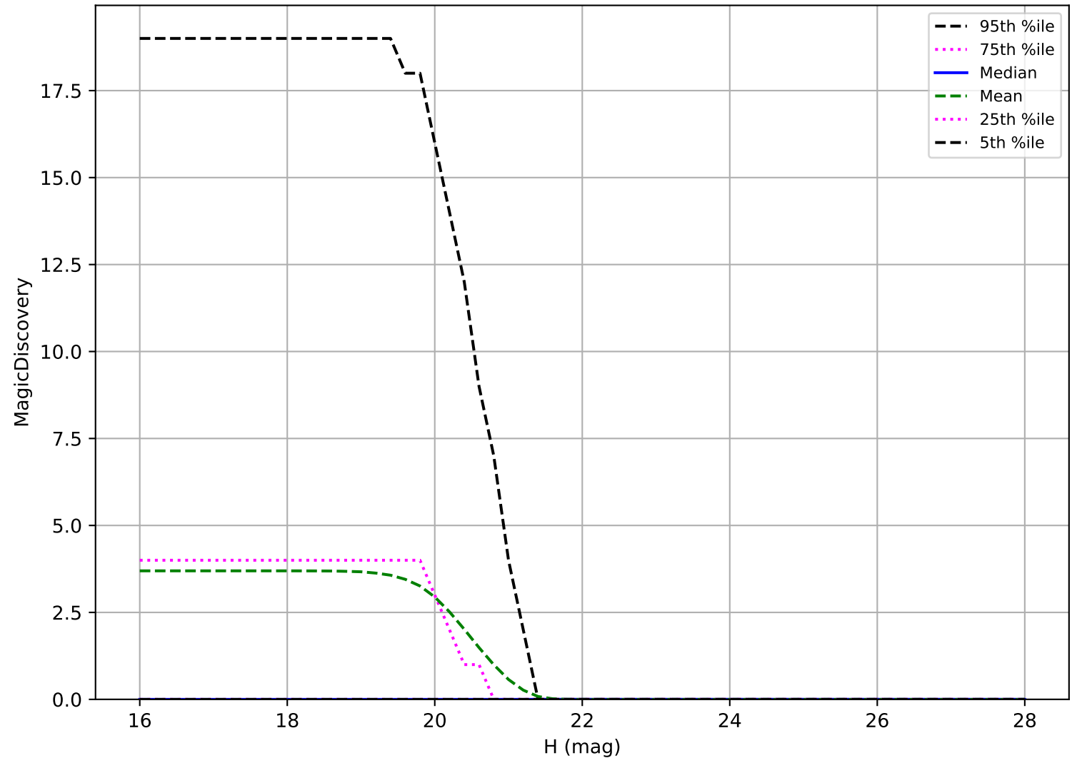
too_elab_heavy_r64_d2_griz_v3.4_10yrs: Vatira 6 detections in 60 nights detection loss
