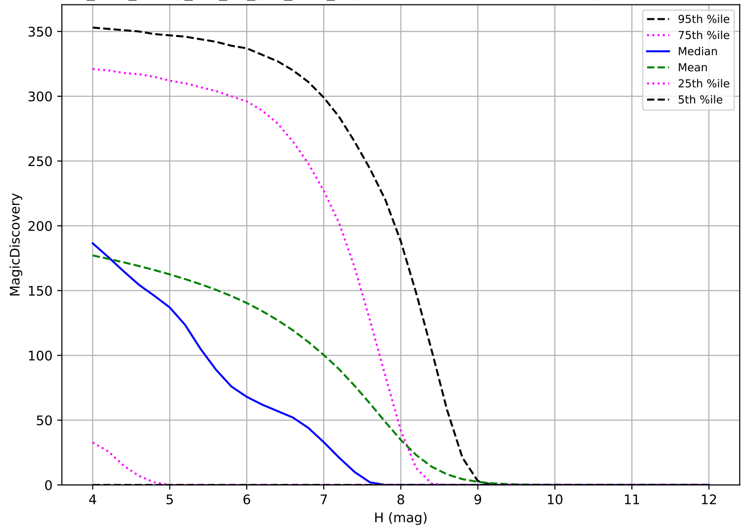
too_elab_heavy_r64_d2_griz_v3.4_10yrs: TNO 6 detections in 60 nights detection loss
